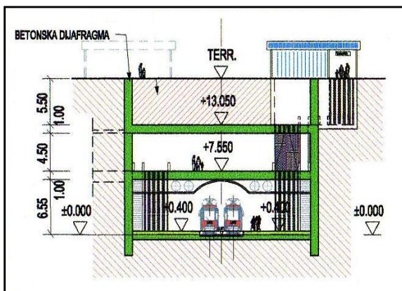
CROSS SECTION OF TOP-DOWN MAIN SQUARE STATION
