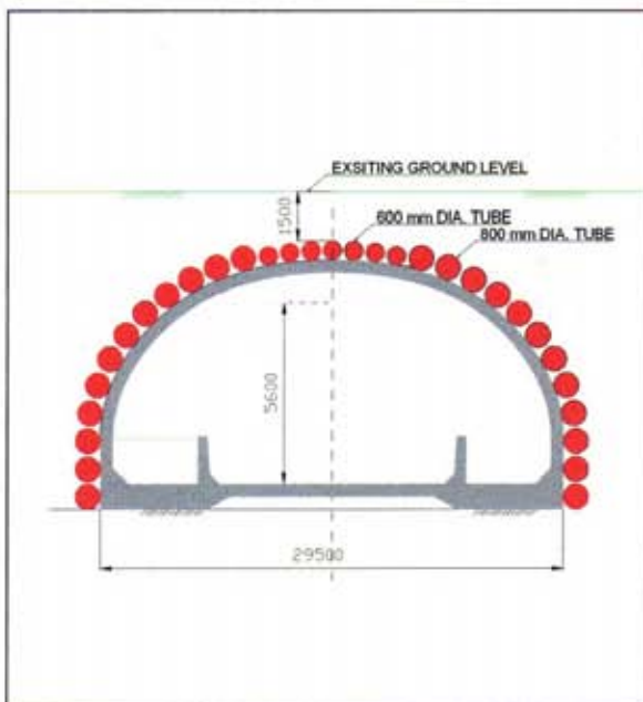
CROSS SECTION
